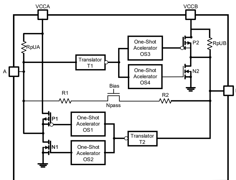
When transmitting data from A-ports to B-ports, during a rising edge the one-shot circuit (OS3) turns on the PMOS transistor (P2) for a short-duration which reduces the low-to-high transition time. Similarly, during a falling edge, when transmitting data from A to B, the one-shot circuit (OS4) turns on the N-channel MOSFET transistor (N2) for a short-duration which speeds up the high-to-low transition. The B-port edge-rate accelerator consists of one-shot circuits OS3 and OS4. Transistors P2 and N2 and serves to rapidly force the B port high or low when a corresponding transition is detected on the A port.
