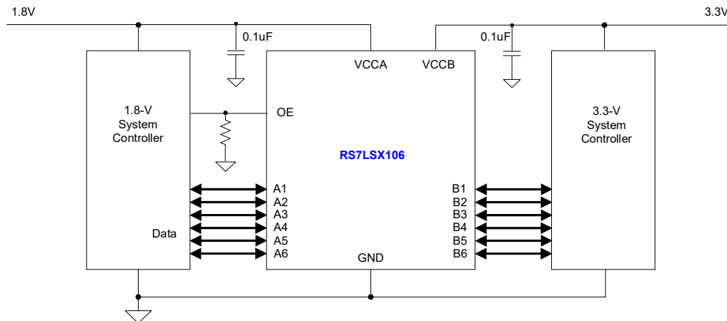
Figure 10 Application Circuit
