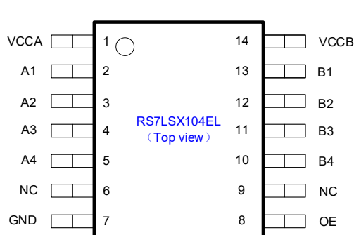
TSSOP14 (Top view)
