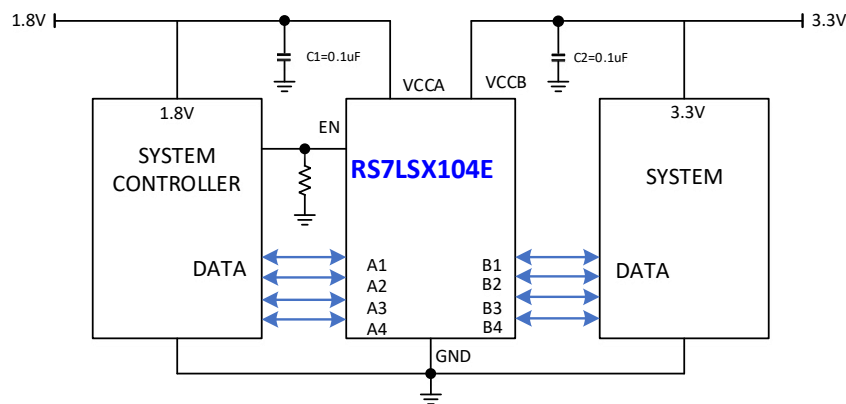
Figure 9 Application Circuit
