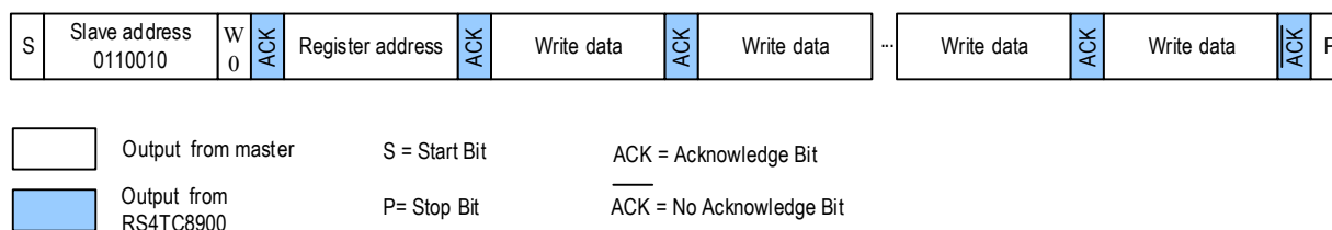
Figure 7 Write Mode Sequence
