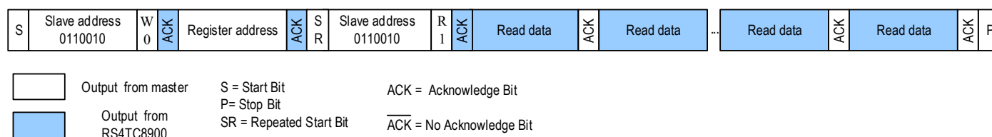
Figure 6 Read Mode Sequence
