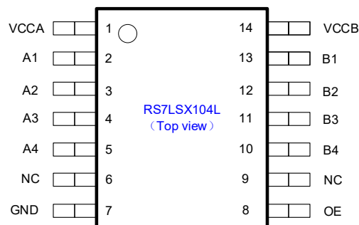
TSSOP14 (Top view)
