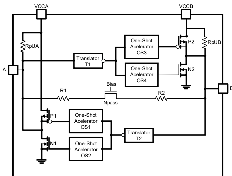
When transmitting data from A-ports to B-ports, during a rising edge the one-shot circuit (OS3) turns on the PMOS transistor (P2) for a short-duration which reduces the low-to-high transition time. Similarly, during a falling edge, when transmitting data from A to B, the one-shot circuit (OS4) turns on the N-channel MOSFET transistor (N2) for a short-duration which speeds up the high-to-low transition. The B-port edge-rate accelerator consists of one-shot circuits OS3 and OS4. Transistors P2 and N2 and serves to rapidly force the B port high or low when a corresponding transition is detected on the A port.
