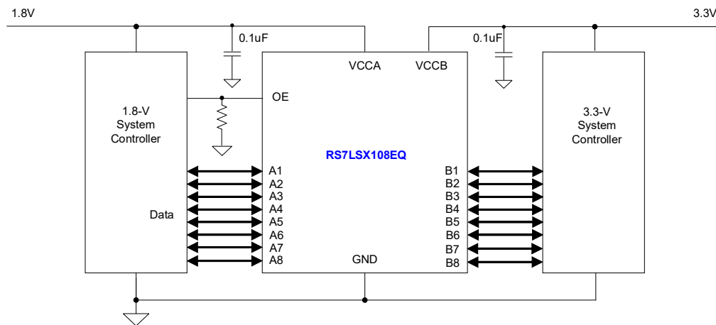
Figure 9 Application Circuit
