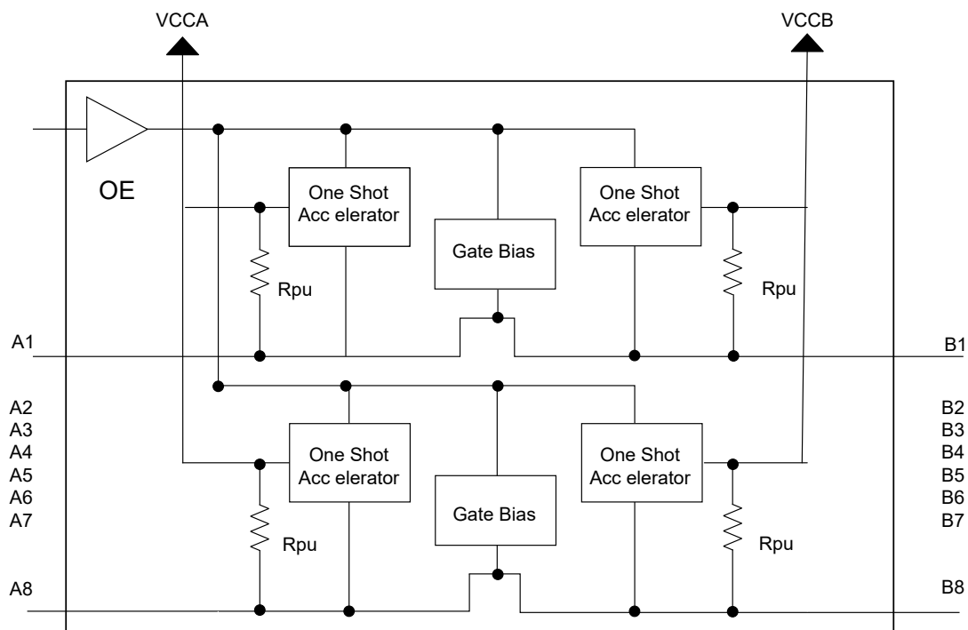
Figure 1: Block Diagram
