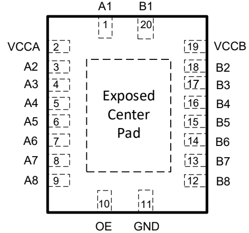
DFN 20 (Top view)
