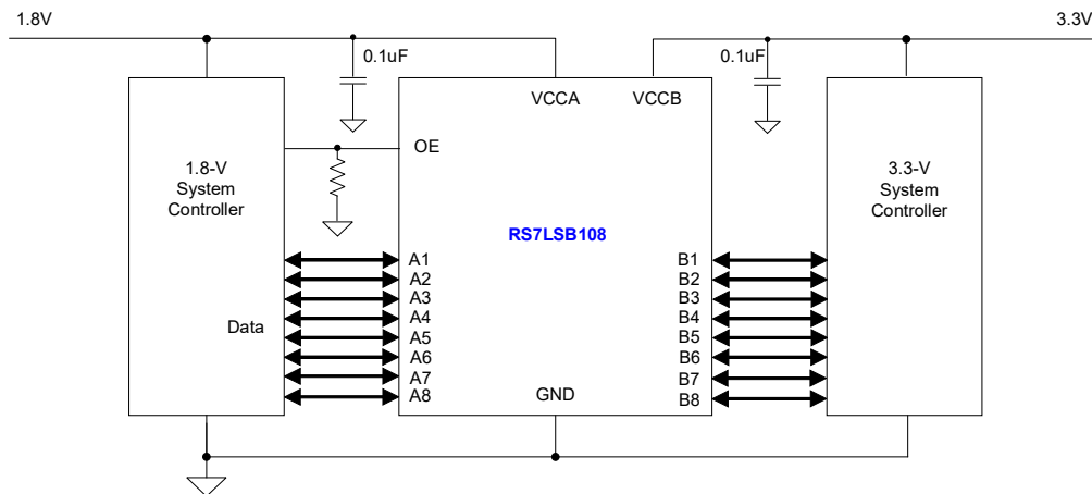
Figure 10 Application Circuit
