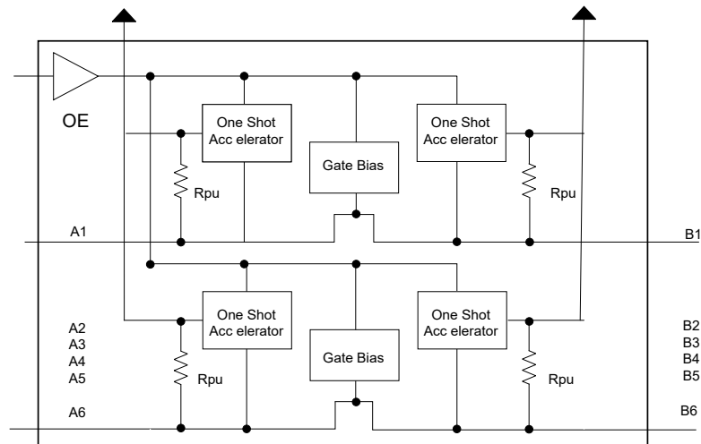
Figure 1: Block Diagram
