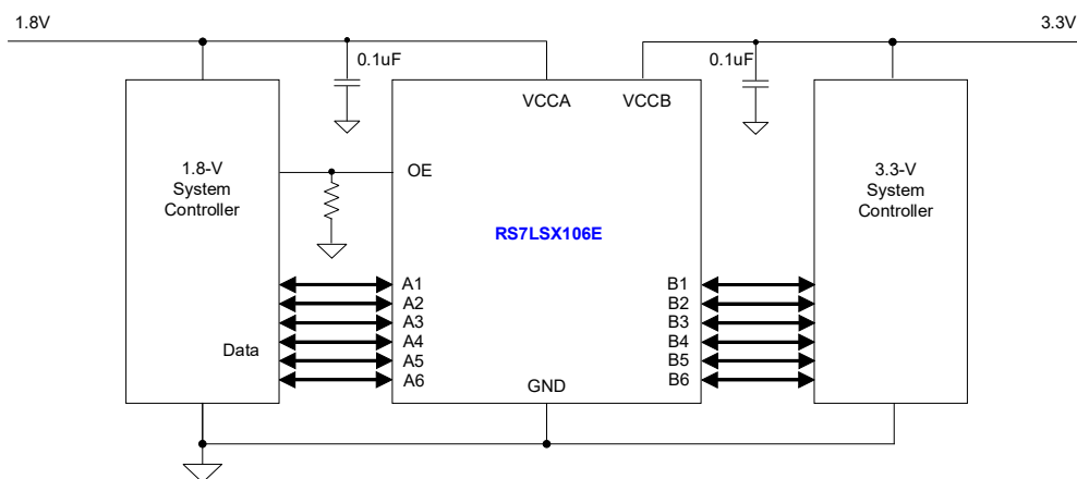
Figure 9 Application Circuit
