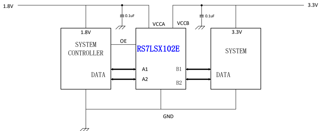
Figure 9 Application Circuit
