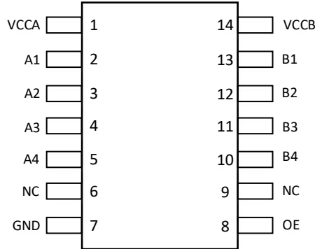
Figure 2 Pin Configuration
