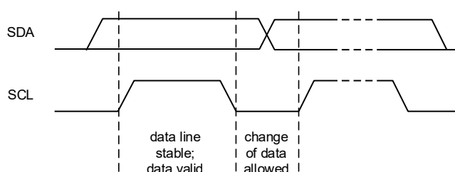
Figure10 Bit transfer
