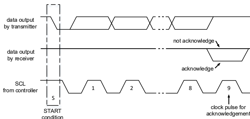
Figure12 Acknowledgement on the IIC bus
