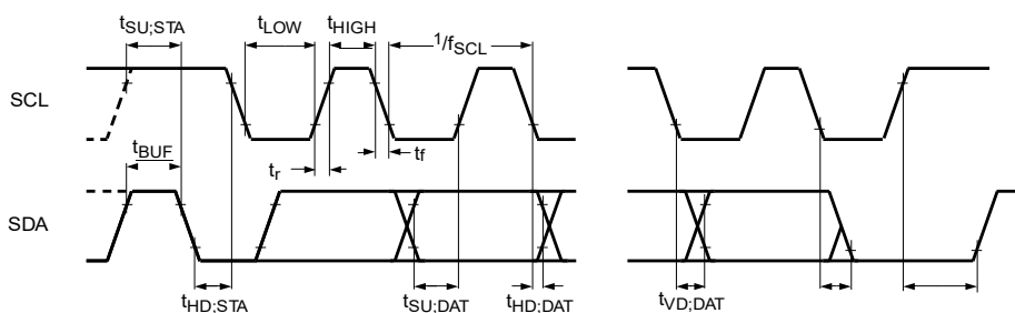
Figure 15. I 2 C-bus timing diagram; rise and fall times refer to 30 % and 70 %
