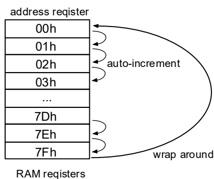
Figure9 SRAM register incrementing
