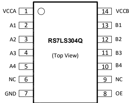
TSSOP-14(Top View)
