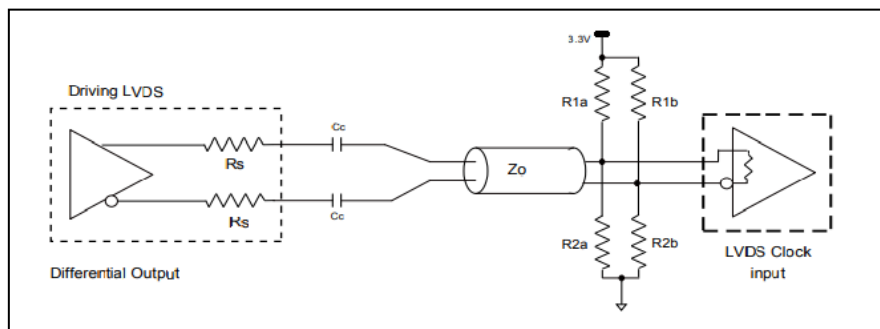
Figure 3. Differential Output Driving LVDS
