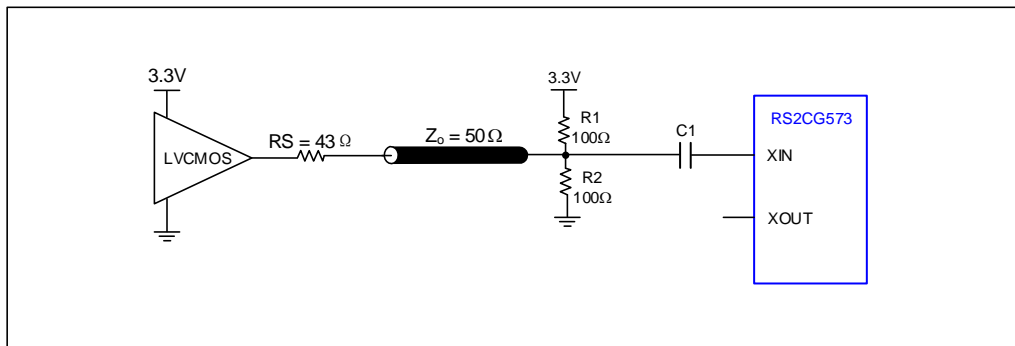
Figure 1A. General Diagram for LVCMOS Driver to XTAL Input Interface
