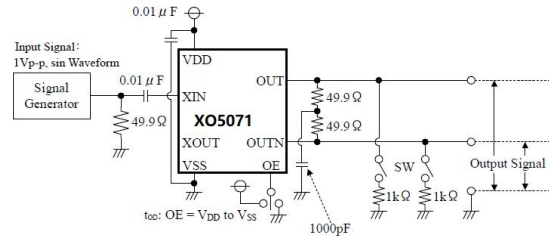
Measurement Circuit 5: t_{OD} , t_{OE}
