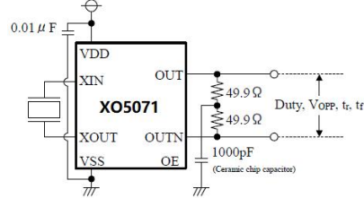
Measurement Circuit 4: Duty, V_{OPP} , t_r , t_f
