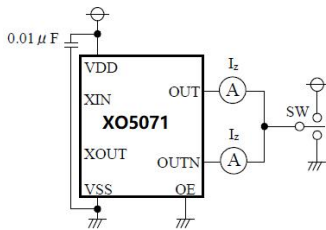
Measurement Circuit 3: I_Z
