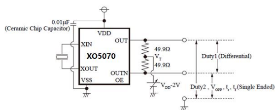
Measurement Circuit 4: Duty1, Duty2, V_{OPP} , t_r , t_f
