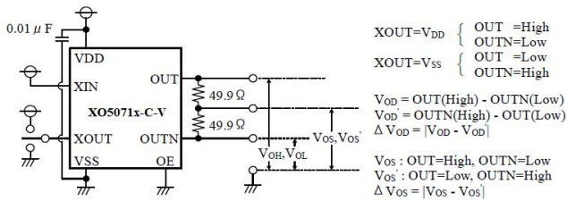
Measurement Circuit 2: V_{OL} , V_{OH}
