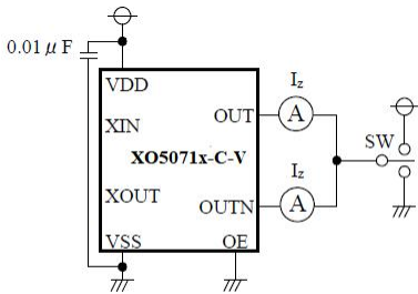
Measurement Circuit 3: I_z
