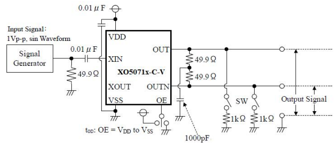
Measurement Circuit 5: t_{op}
