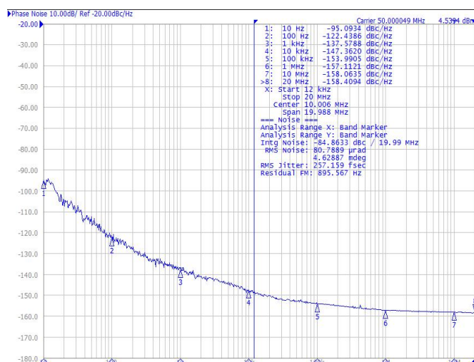
50MHz/15pf/1.8V
