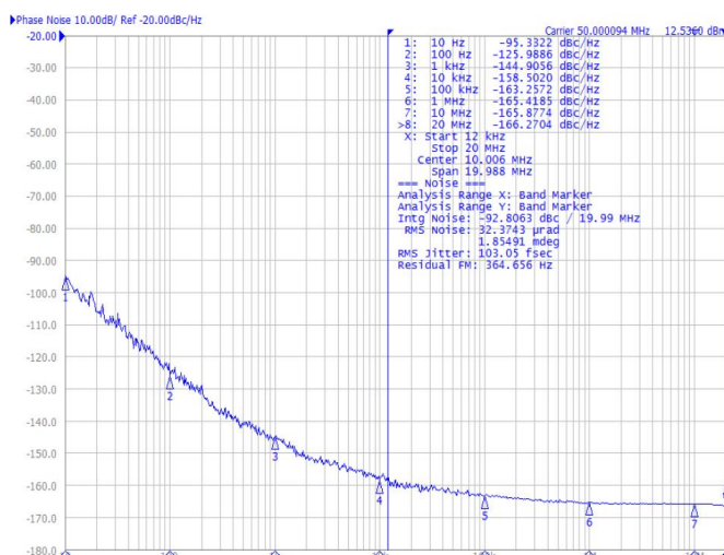
50MHz/15pf/3.3V
