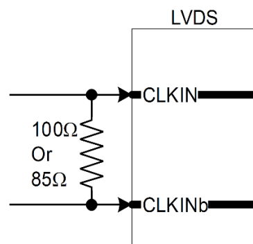
Figure 9. LVDS Input Levels
