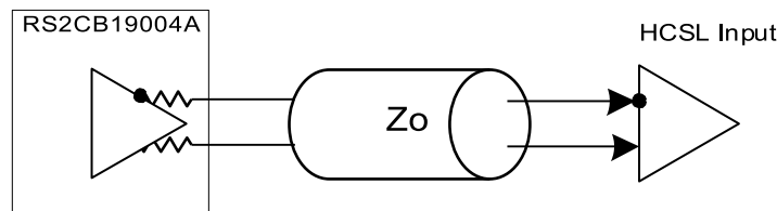
Figure 12. Direct-Coupled Source-Terminated HCSL
