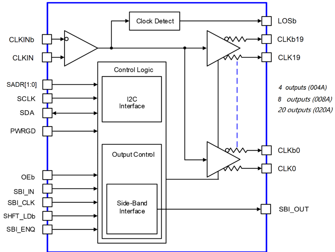
Figure 1. RS2CB19004A/008A/020A Block Diagram
