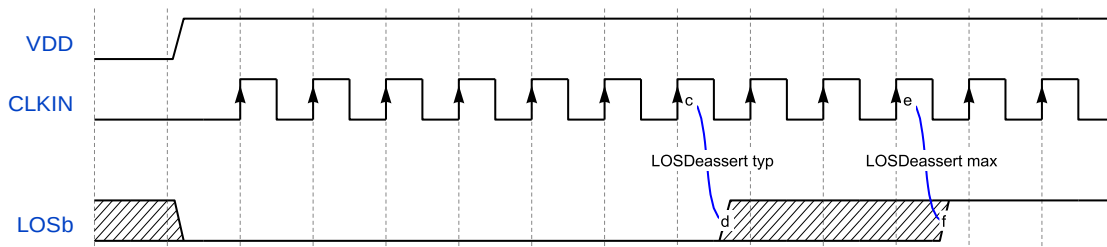
Figure 15. LOSb De-assert Timing RS2CB19004A Devices
