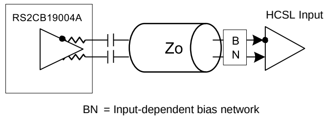
Figure 14. AC-Coupled
