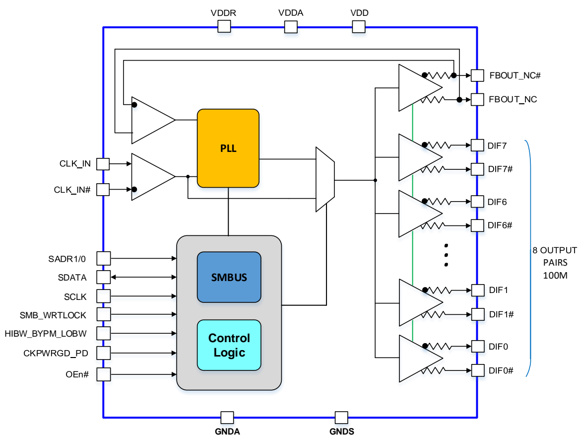
Figure 1. RS2CB2308 Block Diagram
