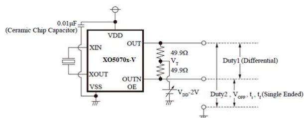
Measurement Circuit 4: Duty, V_{OPP} , t_r , t_f
