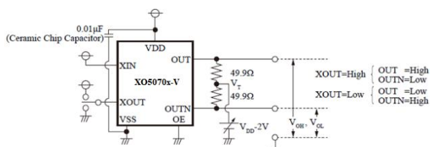
Measurement Circuit 2: V_{OL} , V_{OH}
