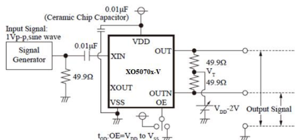
Measurement Circuit 5: t_{OD} , t_{OE}
