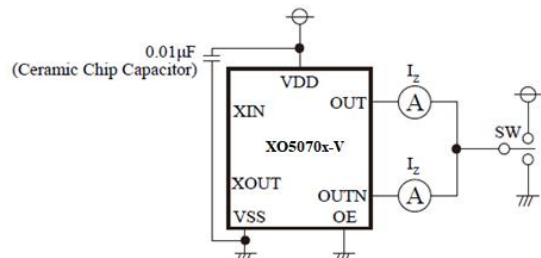
Measurement Circuit 3: I_z
