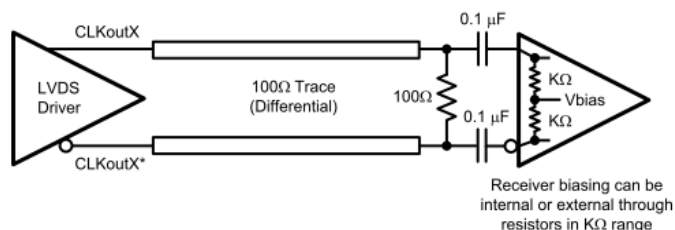
Differential LVDS Operation With AC Coupling to Receivers Without Internal 100Ω Termination
