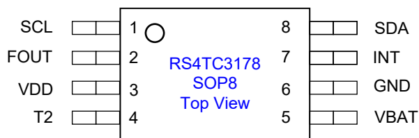
RS4TC3178S SOP8
