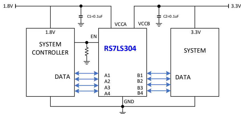
Figure 7. Typical Application
