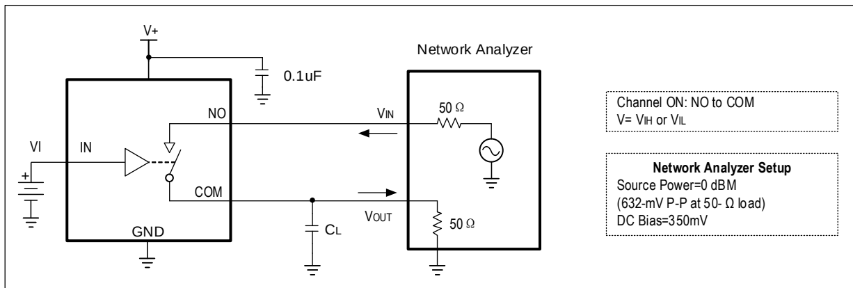
Figure 7、Bandwidth (BW)
