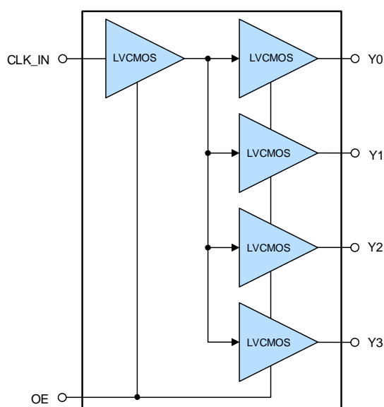
Figure 1 Block Diagram
