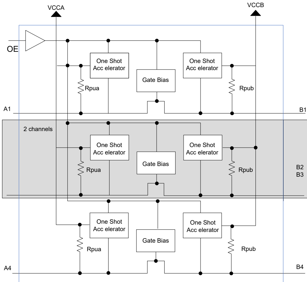
Figure 1. RS7LS104AQ block diagram
