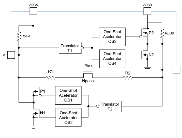
Figure 9. Architecture of a RS7LS104AQ Cell
