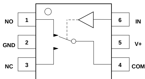
RS3SW2157 SOT23-6, Top View
