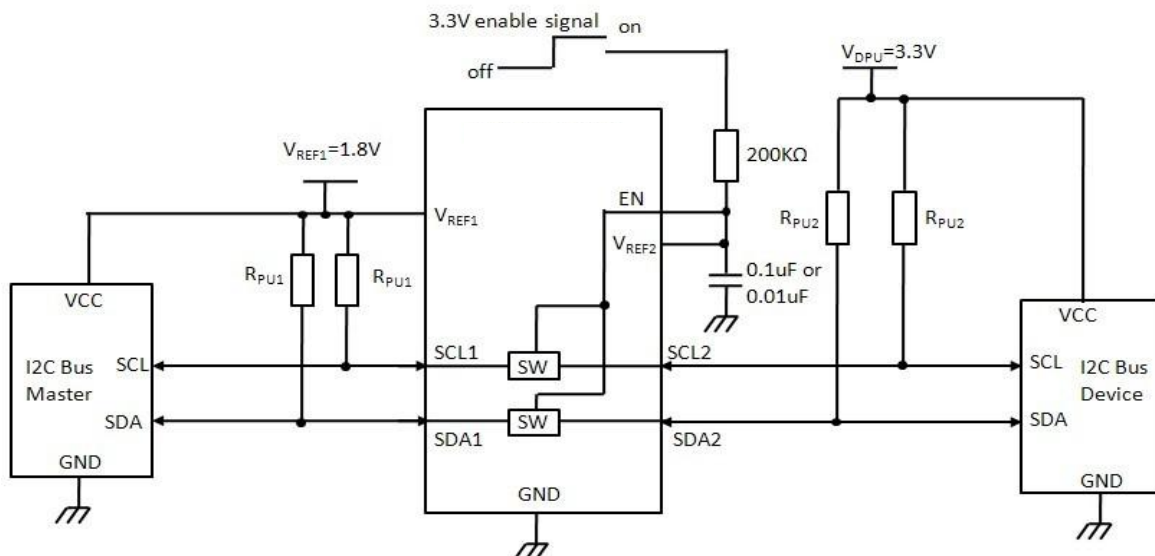
Figure 4 Typical Open Drain Application Circuit (Switch Enabled Control)
