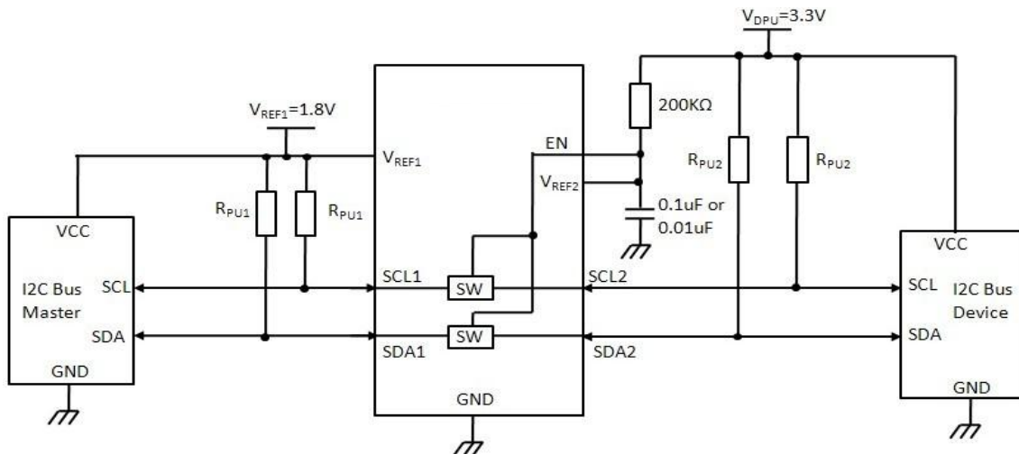
Figure 3 Typical Open Drain Application Circuit (Switch Always Enabled)
