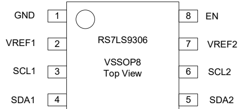
VSSOP8(Top view)
