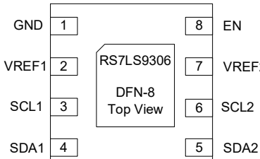
DFN-8 (Top view)
