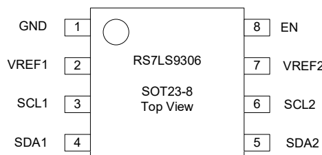
SOT23-8(Top view)
