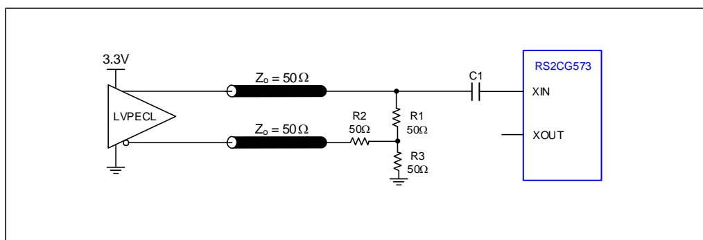
Figure 1B. General Diagram for LVPECL Driver to XTAL Input Interface
