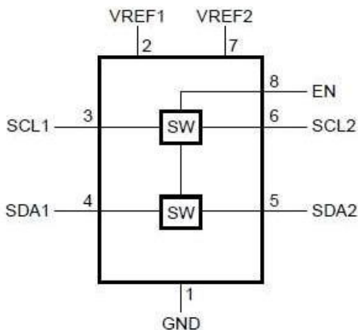
Figure 1: Block Diagram
