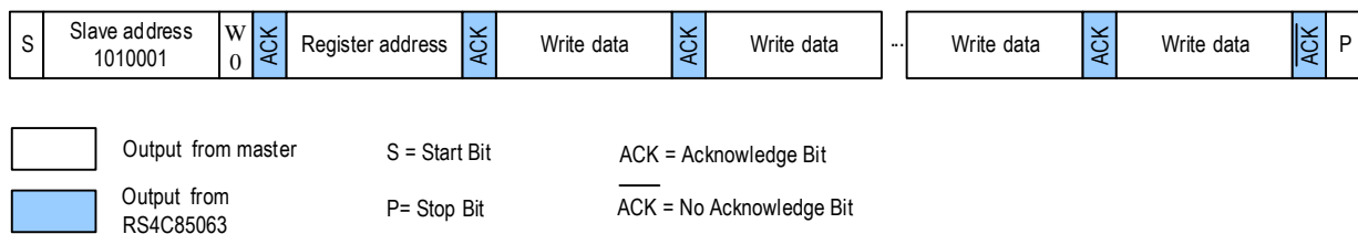
Figure10 Write Mode Sequence
