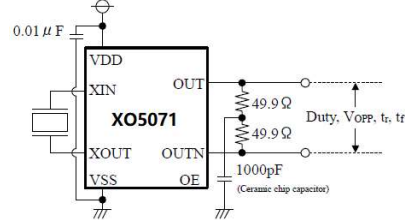
Measurement Circuit 4: Duty1, Duty2, V OPP , t r , t f
