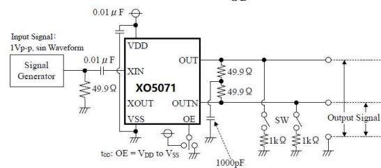
Measurement Circuit 5: t OD
