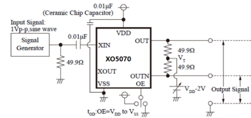
Measurement Circuit 5: t_{OD} , t_{OE}
