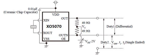
Measurement Circuit 4: Duty, V_{OPP} , t_r , t_f
