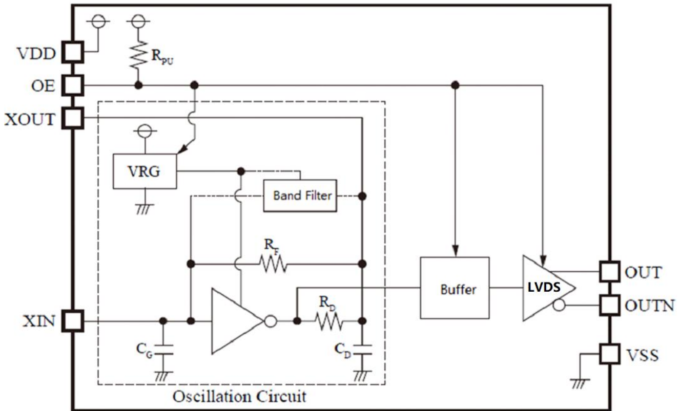
Figure 1 XO5071x Block Diagram
