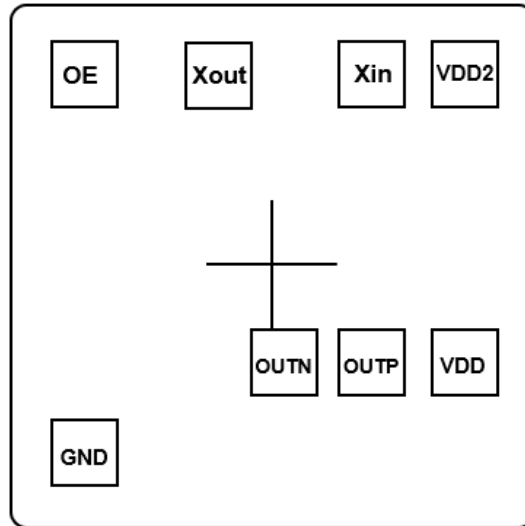
Figure 2 Pin Configuration
