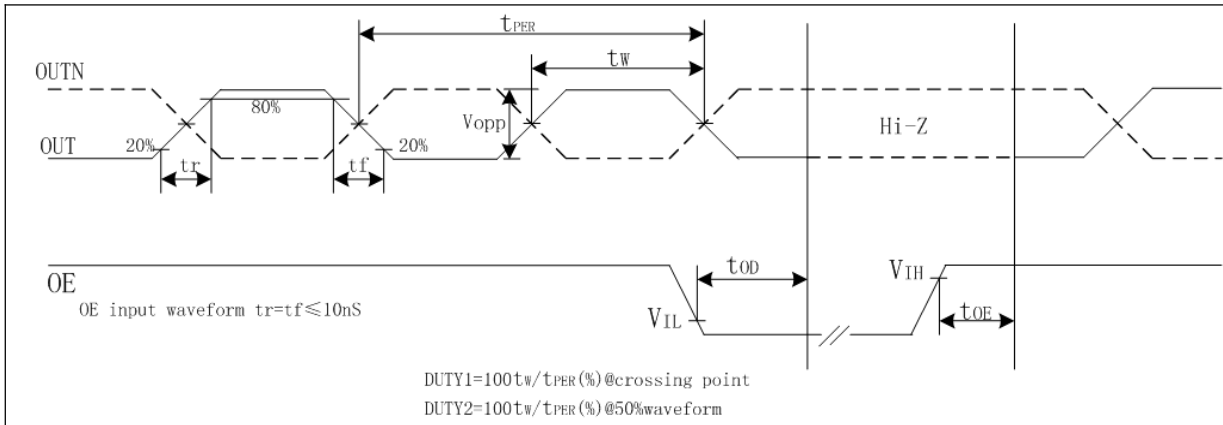
Figure 3 Timing chart
