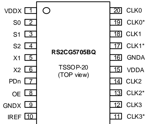
Figure 2 Pin Configuration
