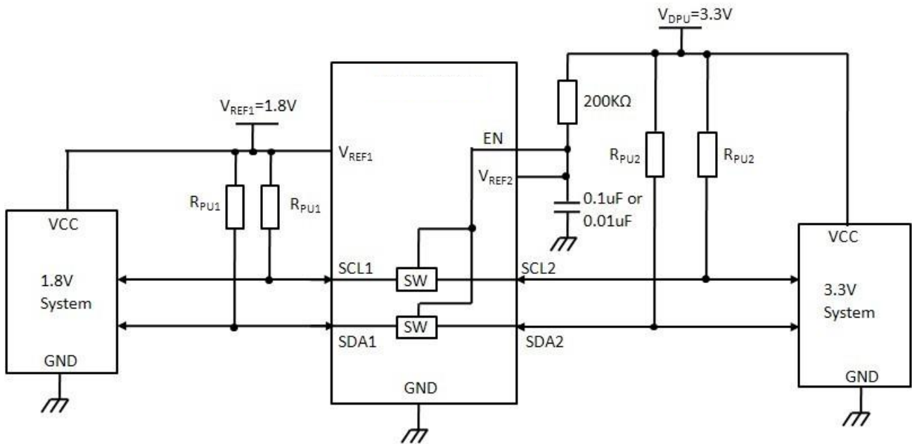
Figure.5 Typical push-pull Application Circuit (Switch Always Enabled)
