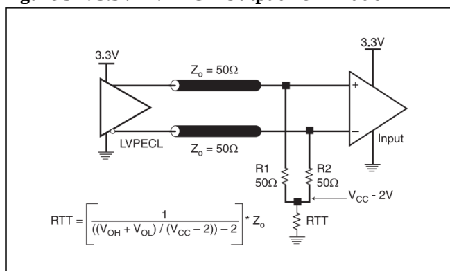
Figure 3A. 3.3V LVPECL Output Termination
