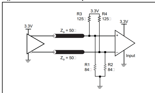
Figure 3B. 3.3V LVPECL Output Termination
